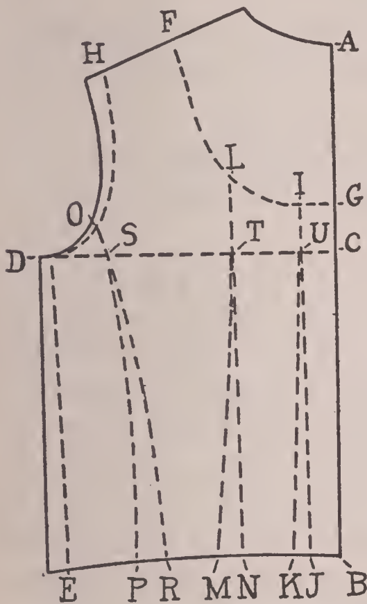
Fig. (29) Diagram for back of brassiere
